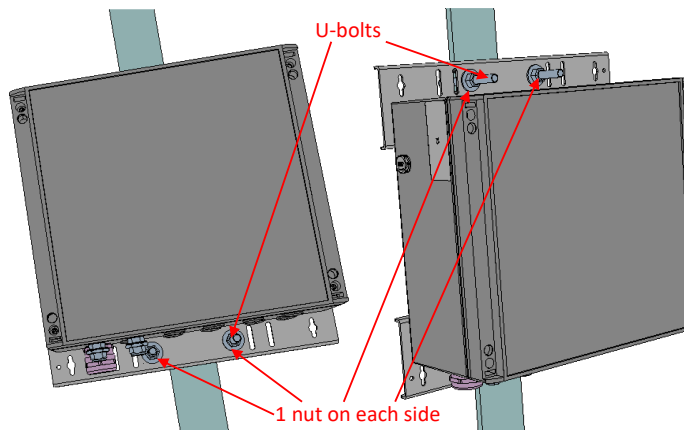
To screw the U-bolts, it is recommended to use the four nuts provided in the mounting kit.
