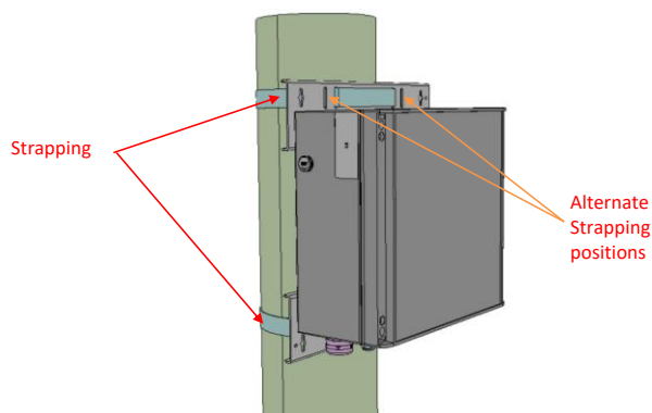
Metallic strapping mounting with maximum acceptable width of 25mm
