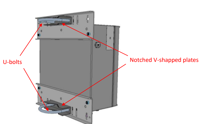
The Wirnet™ iBTS is delivered with two notched V-shaped plates and two U-bolts to be mounted on a pole with a maximum diameter of 60mm
